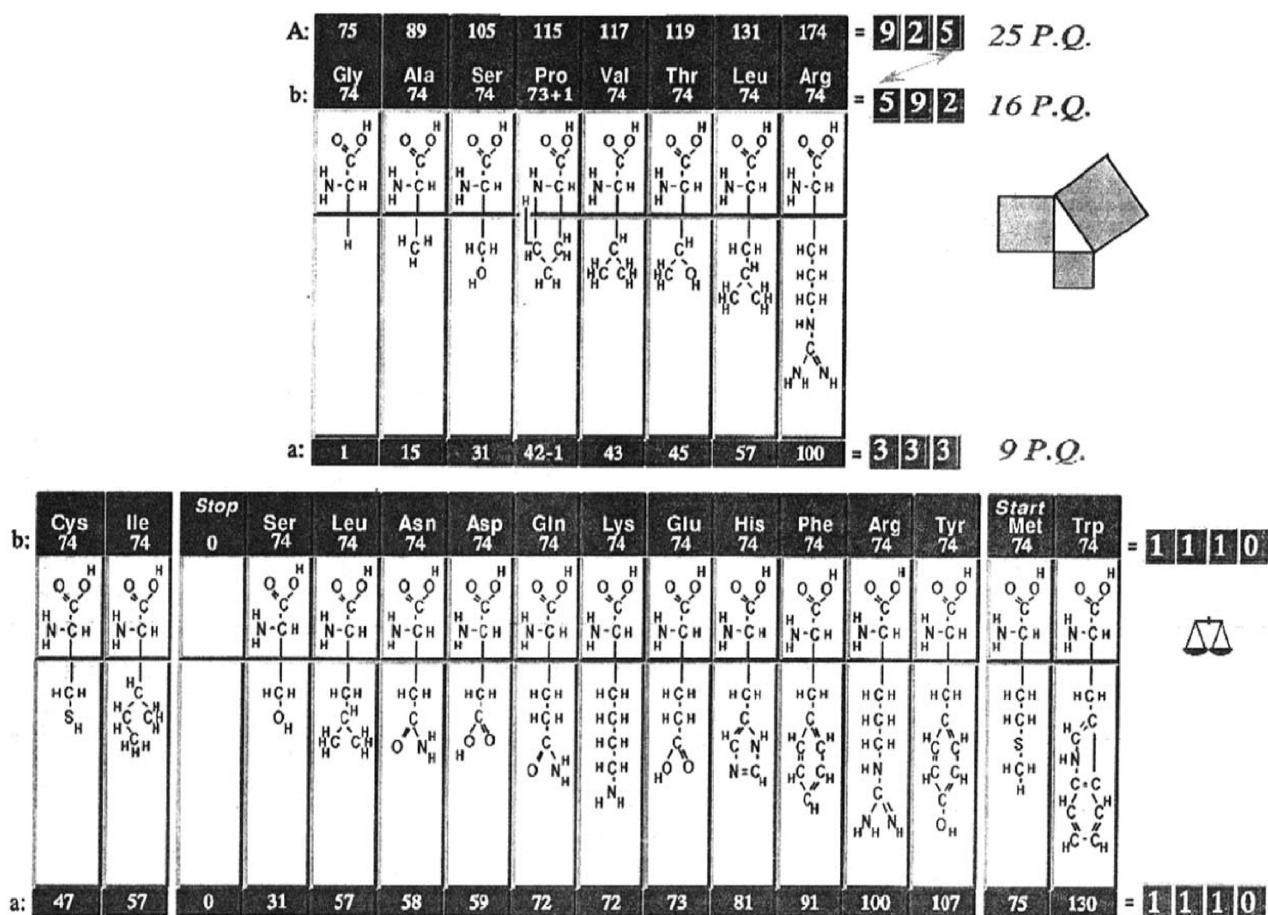
Fig. 2. Algebraic group correlations between atomic masses of amino acids. Here PQ = 37 . ( PQ = Prime Quantum, printed by courtesy of Shcherbak).
