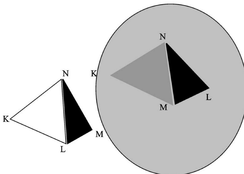
Fig. 3. Tetrahedron (left) and its mirror image (right).
